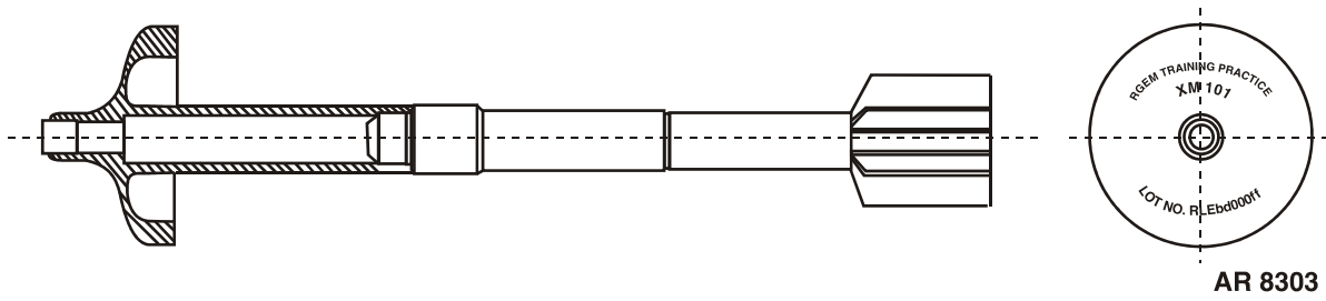
Figure 1-4a. Grenade, Rifle, Entry Munition, Target Practice, M101
