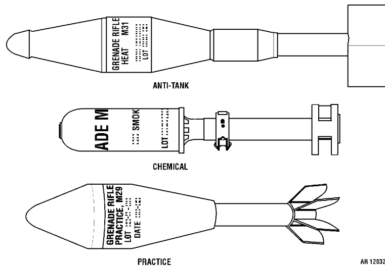
Figure 1-4. Representative types of rifle grenades.
