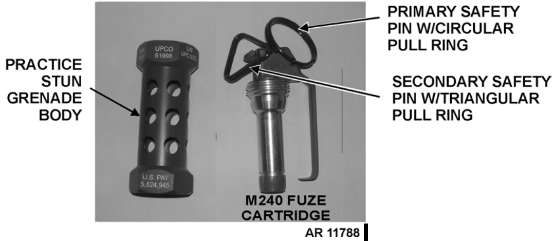
Figure 2-5.1. Components of M102 Reloadable Stun Practice Hand Grenade: Practice Stun Grenade Body and M240 Fuze Cartridge.
