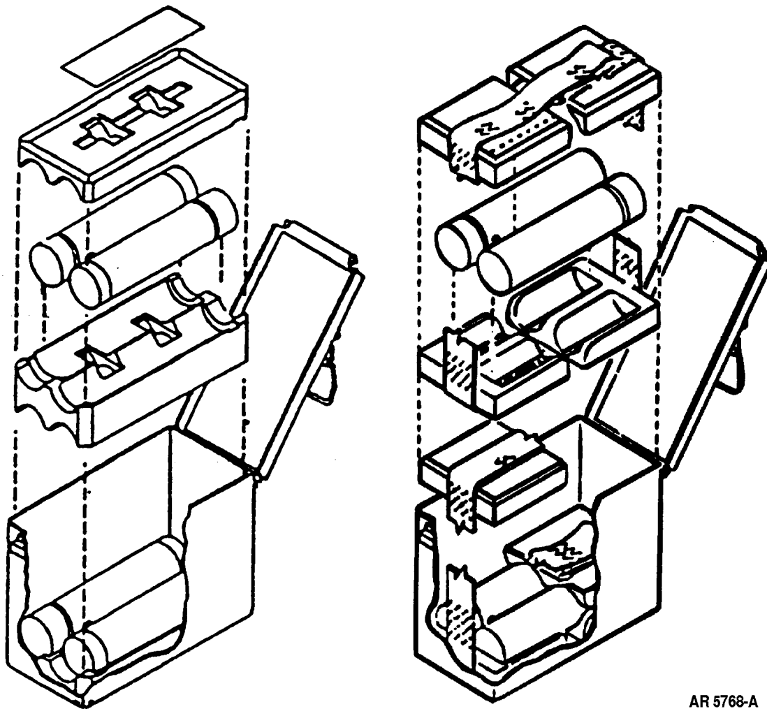
Figure 3-3.2. IR, simulant, anti-riot, and non lethal grenade boxes and packing.
