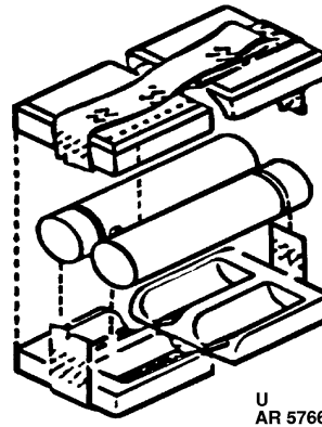
Figure 3-11.1. Grenade/spacer assembly
